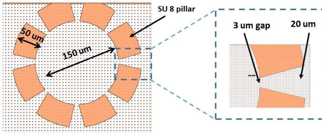
Figure 1: During the time of installation, vendor must demonstrate fabrication of this design on SU8. The design comprised of SU8 pillars arranged in a circular manner. Importantly the minimum separation between the pillars is 3 micrometers. The pillar height is 30 micrometers.
